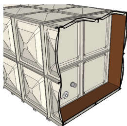
Sectional Elevation
